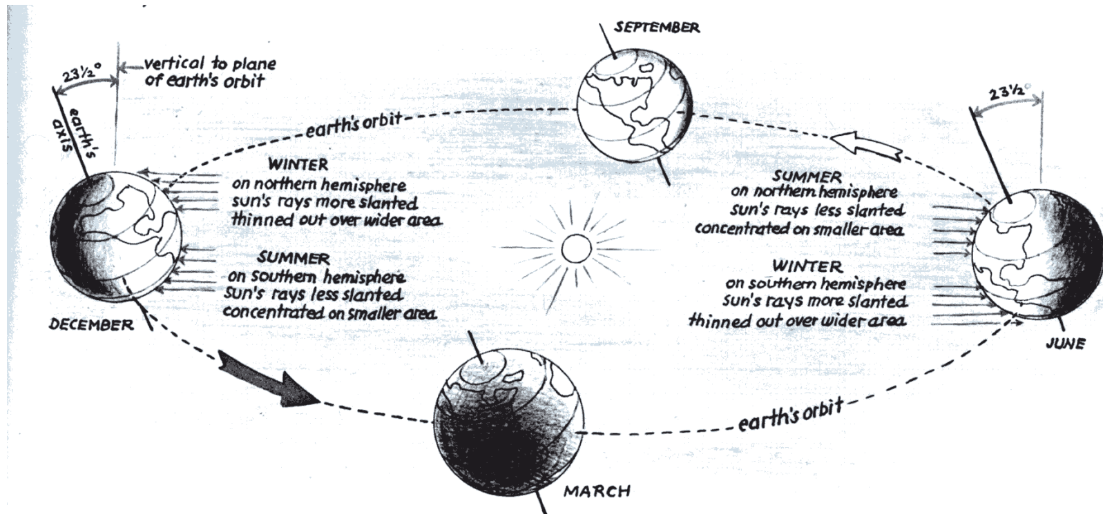
Figure 21: Tilt of Earth's Axis Causes the Seasons
