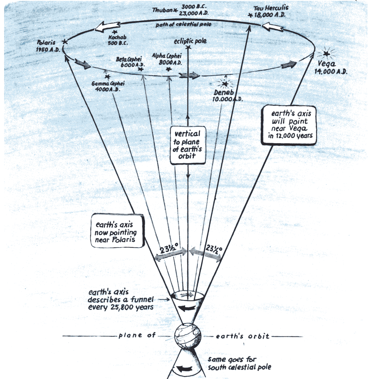
Figure 24: The Wobble of the Earth's Axis
